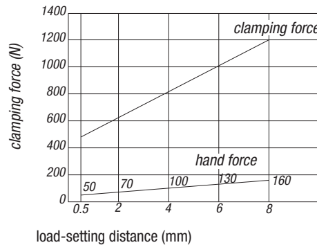
Swing Clamps K0912....4540
