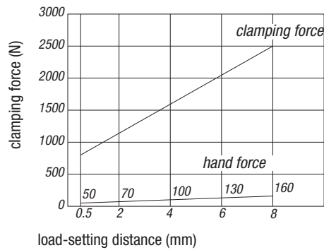
Pull Clamps K0910.4050...
